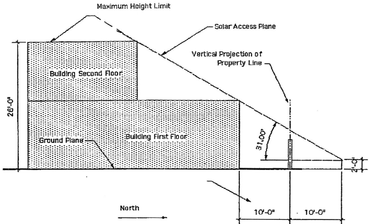
Building Cross-Section Indicating Solar Access Angle at North Property Line
